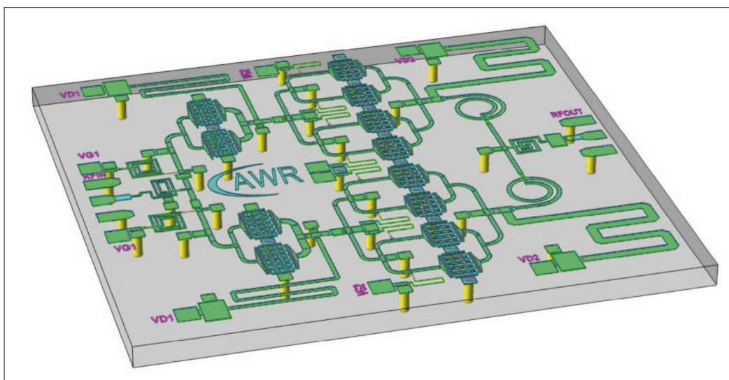
Figure 4: 3D layout view of the designed MMIC amplifier
