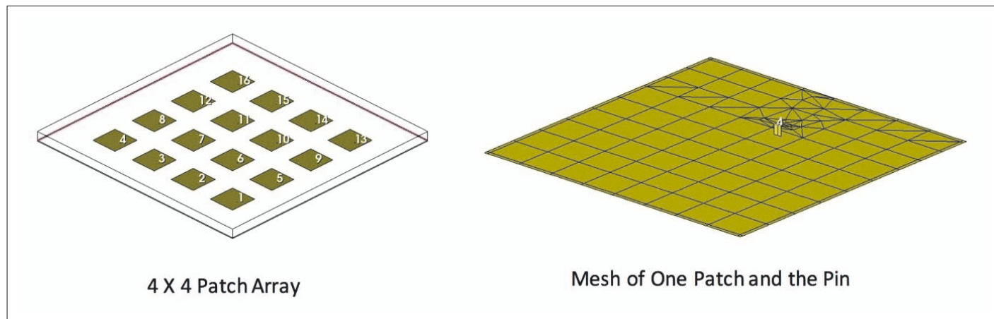
Figure 1: A 4x4 patch array (left), where each patch is fed by a pin coming up from the bottom ground plane. The right picture shows the mesh of one element, and the driving pin to the ground plane
