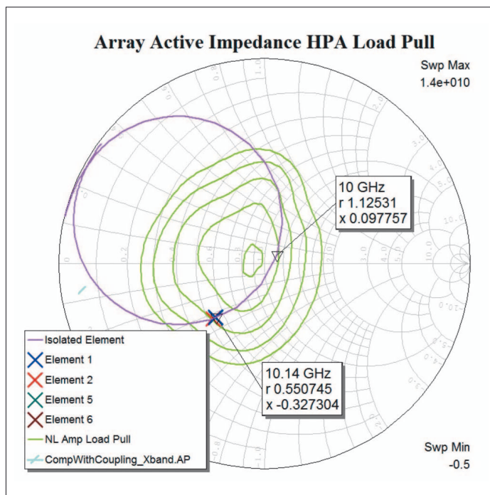
Figure 5: The Smith chart shows the Input impedance to an isolated element and to elements when the entire array is simulated. Load pull contours for power getting to the load are also shown
