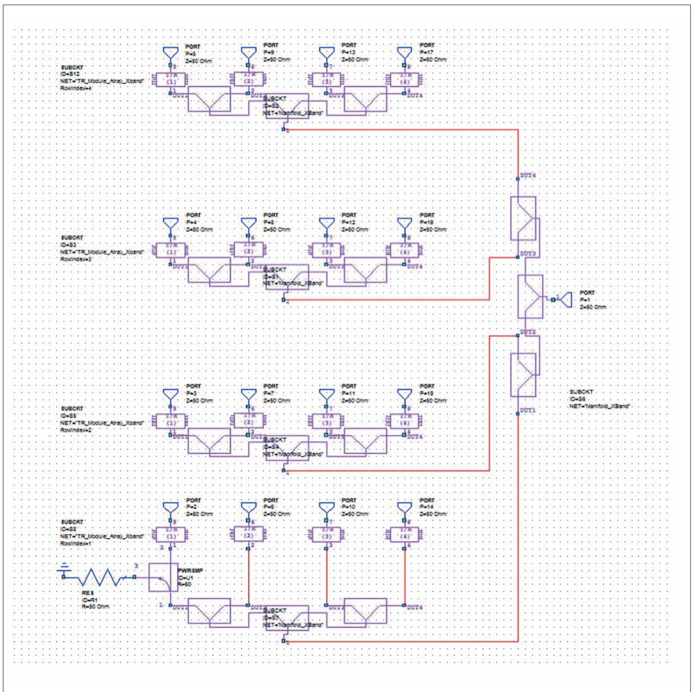
Figure 2: Corporate feed network for the patch array. Each element is driven by a MMIC amplifier, and controlled by a phase shifter and attenuator
