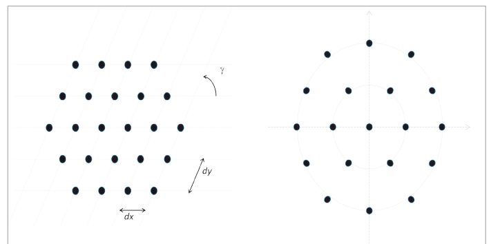
Figure 9: VSS standard array geometries: lattice (left) and circular (right)
