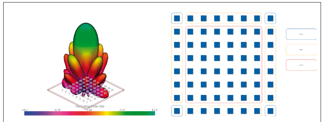
Figure 8: The coupling elements for center edges, and corners of the array (left) and resulting EM Simulation (right 9)
