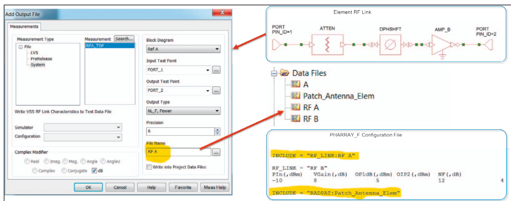
Figure 4: VSS phased-array element with RF link characterization
