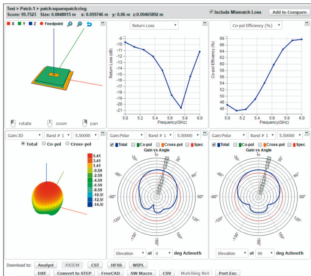
Figure 7: An ArtiSyn antenna pattern file can be imported into the VSS phased array model
