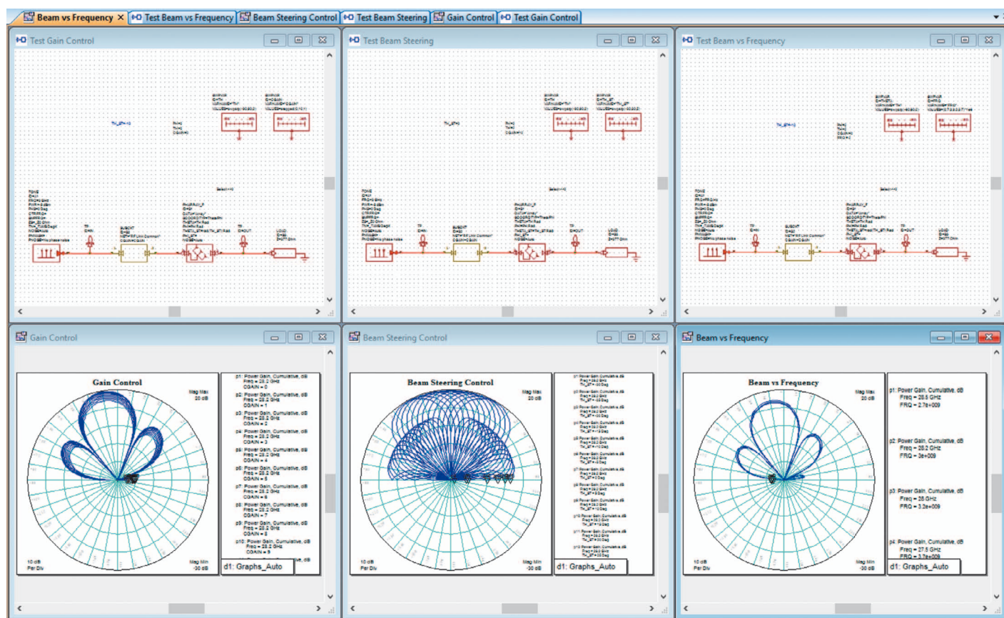
Figure 15: 28-GHz-phased-array transceiver in VSS-Software
