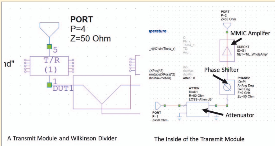
Figure 3: The picture shows one Wilkinson divider and the transmit module, which contains the phase shifter, attenuator, and a MMIC amplifier
