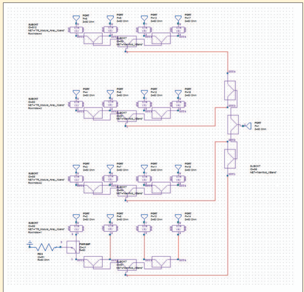
Figure 2: Corporate feed network for the patch array. Each element is driven by a MMIC amplifier, and controlled by a phase shifter and attenuator
