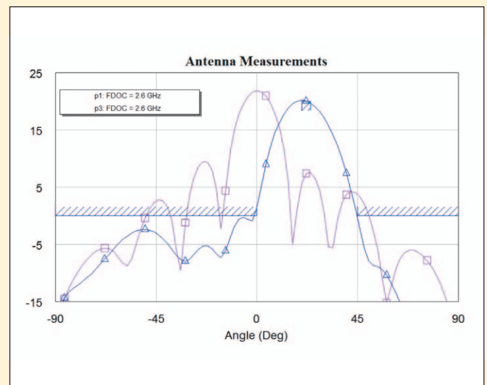
Figure 7: The antenna pattern is optimized to be below the blue bars
