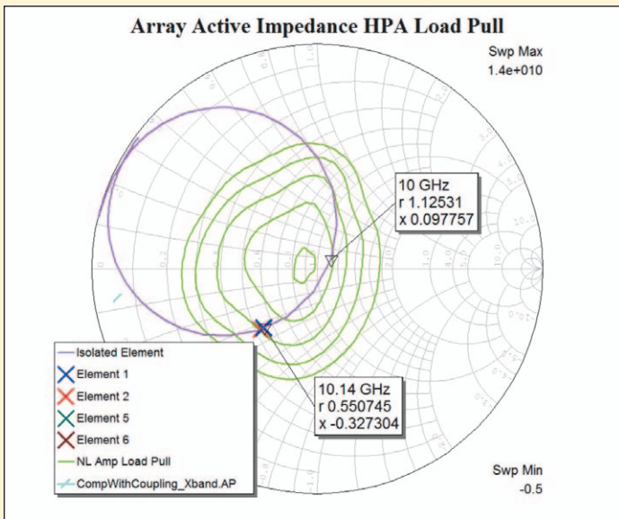
Figure 5: The Smith chart shows the Input impedance to an isolated element and to elements when the entire array is simulated. Load pull contours for power getting to the load are also shown
